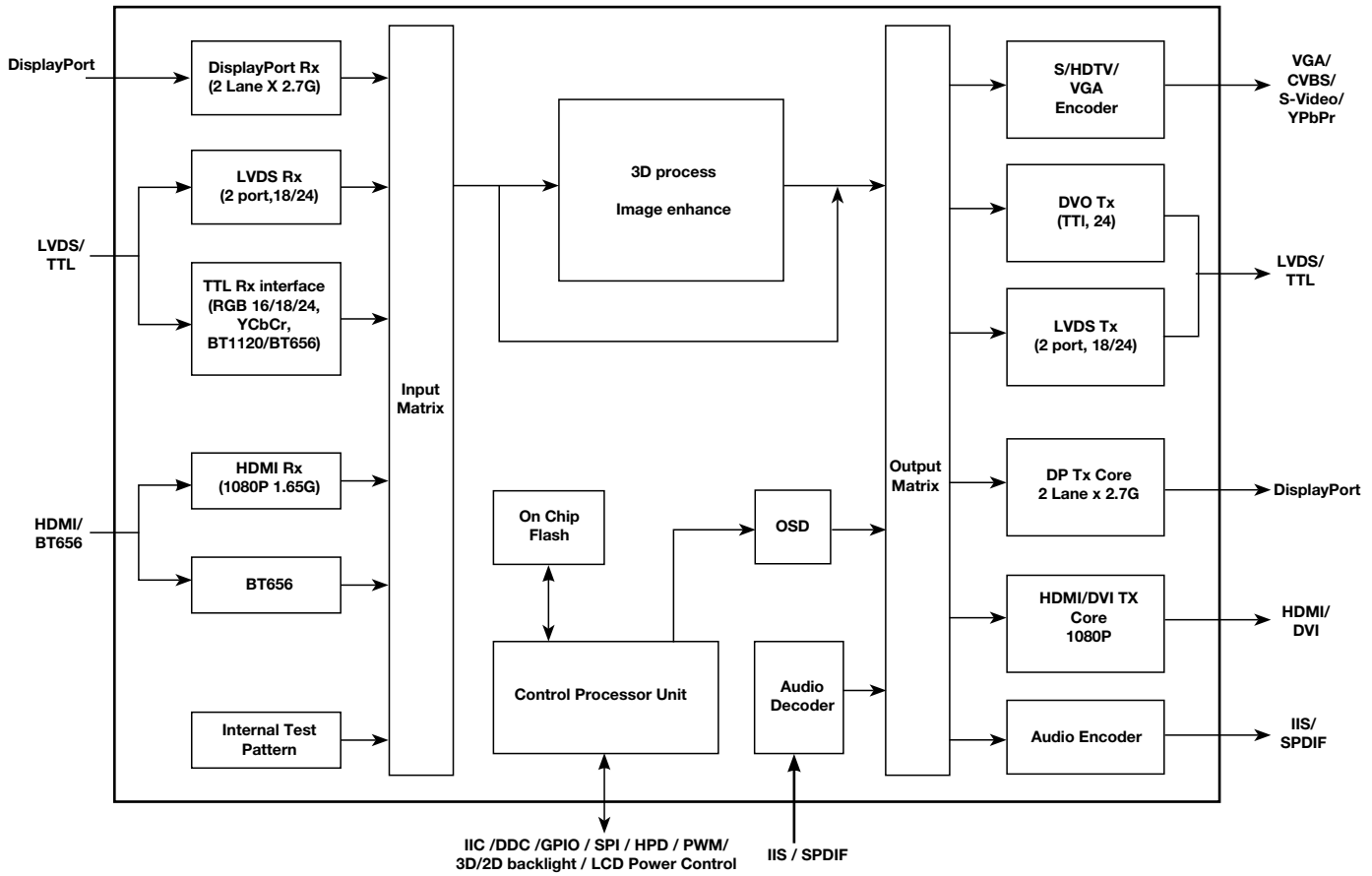
CH7039 Functional Block Diagram
