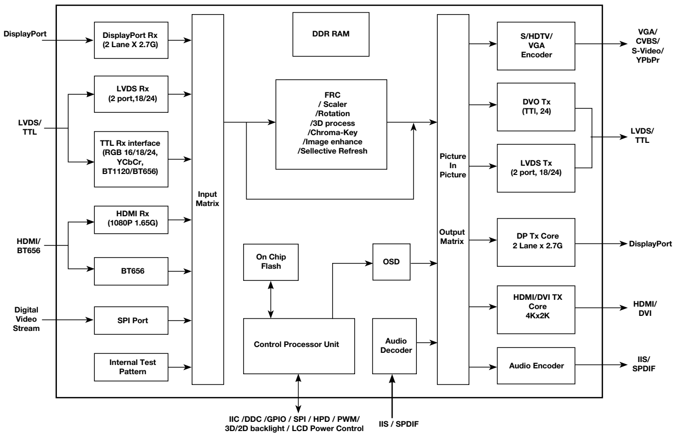
CH7038 Functional Block Diagram
